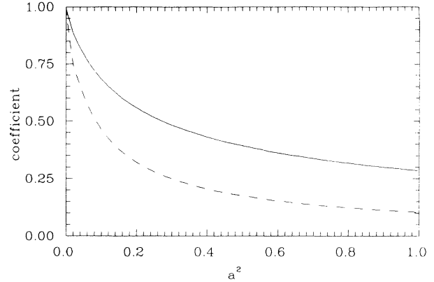
FIG. 1. Shear rate dependence of the self-diffusion coefficient (solid line) D(a) . The same for \Omega(a) (dashed line).
