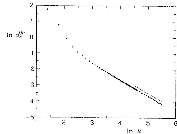
Fig. 2. Log-log plot of a_c^{(k)} versus k . The straight line has a slope equal to -1 .
