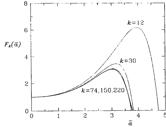
Fig. 3. Scaled determinant F_k(\bar{a}) = \Delta_k(a)/\Delta_k(0) as a function of the scaled shear rate \bar{a} = ka for k = 12, 30, 74, 150 and 220 .
