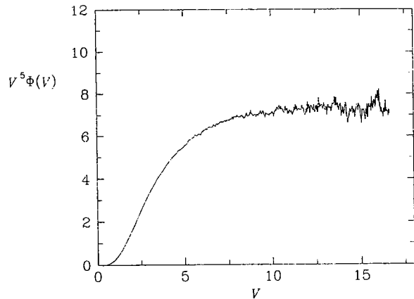
Fig. 5. Plot of V^5\phi(V) for a = a_c^{(4)} \simeq 5.847 .
