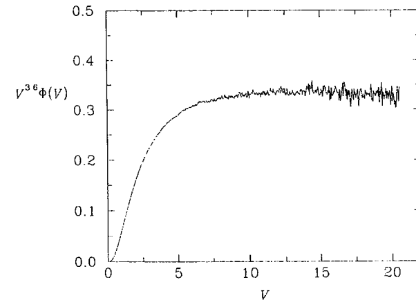
Fig. 7. Plot of V^{3.6}\phi(V) for a = 12 .
