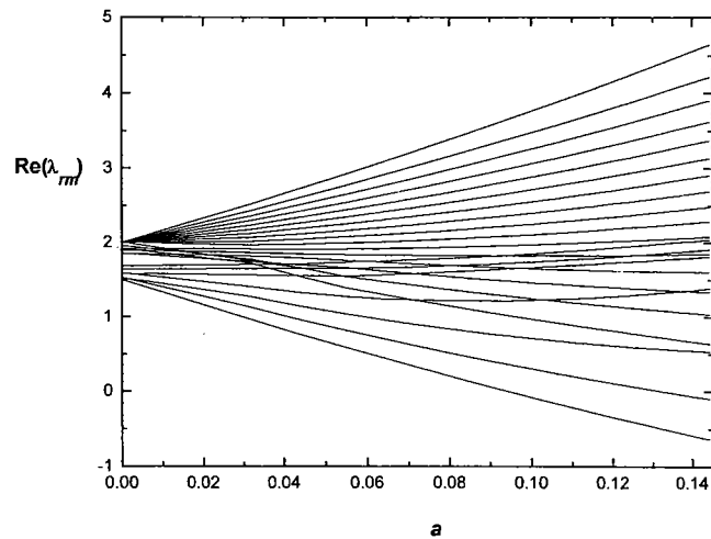
Fig. 1. Shear-rate dependence of the real part of the eigenvalues corresponding to the moments of degree 2r + |m| = 40 .
