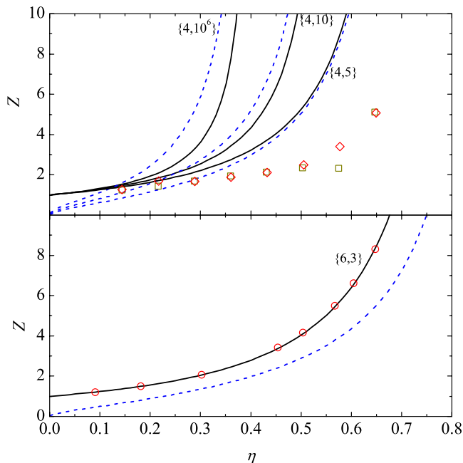
FIG. 1. (Color online) Top panel: Compressibility factor Z as a function of \eta for the isostatic \{4,10^6\} , \{4,10\} , and \{4,5\} tessellations ( |K|^{1/2}\sigma=1.7628 , 1.6169 , and 1.0613 and \eta_{\max}=0.4142 , 0.5750 , and 0.7206 , respectively); solid lines: Eq. (1); dashed lines: free area theory of Ref. 3; the symbols are simulation results also obtained in Ref. 3 for |K|^{1/2}\sigma=1.060 (squares) and |K|^{1/2}\sigma=1.062 (diamonds). Bottom panel: Compressibility factor Z as a function of \eta for the (Euclidean) hexagonal \{6,3\} tessellation ( |K|^{1/2}\sigma=0 , \eta_{\max}=\sqrt{3}\pi/6 ); solid line: Eq. (1); dashed line: free area theory of Ref. 3; the symbols are the simulation results from Ref. 7.
