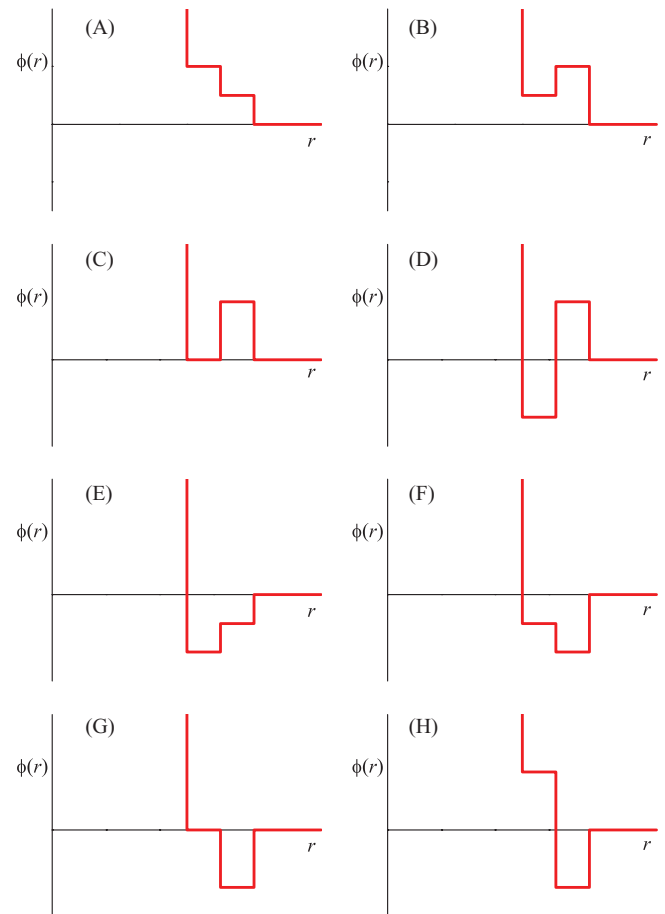
FIG. 1. Diagrams of the surveyed potentials, labeled from A to H.
