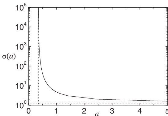
Fig. 2. Plot of the exponent \sigma as a function of the shear rate a . The vertical and horizontal dotted lines indicate the locations of a_{\text{th}} \simeq 0.3520 and \sigma_{\min} \simeq 1.252 , respectively.
