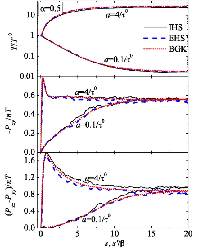
FIG. 8. (Color online) Evolution of T/T^0 , -P_{xy}/nT , and (P_{xx} - P_{yy})/nT for IHS (solid lines) and EHS (dashed lines) in the cases \alpha=0.5 with a\tau^0=0.1 and a\tau^0=4 . The dotted lines are the predictions obtained from the solution of a BGK model. The data have been obtained starting from the initial distribution function (3.12).
