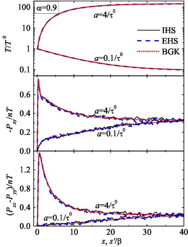
FIG. 7. (Color online) Evolution of T/T^0 , -P_{xy}/nT , and (P_{xx} - P_{yy})/nT for IHS (solid lines) and EHS (dashed lines) in the cases \alpha=0.9 with a\tau^0=0.1 and a\tau^0=4 . The dotted lines are the predictions obtained from the solution of a BGK model. Note that in the top panel the curves corresponding to IHS, EHS, and BGK are practically indistinguishable. The data have been obtained starting from the initial distribution function (3.12).
