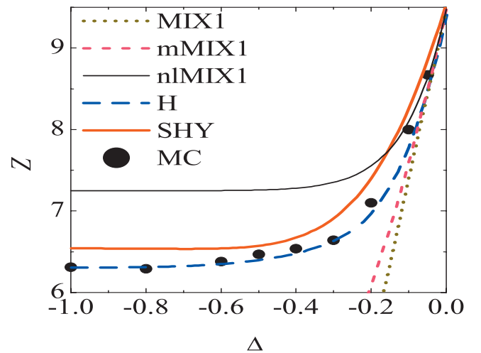
FIG. 8. Plot of the compressibility factor Z vs the nonadditivity parameter \Delta for an equimolar asymmetric binary mixture of nonadditive hard spheres with size ratio \sigma_2/\sigma_1 = \frac{1}{3} at \eta = 0.5 . The dotted line corresponds to the original MIX1 theory, Eq. (3.3), the short-dashed line corresponds to the mMIX1 theory, Eq. (3.3) with Y_{ij}^M \rightarrow Y_{ij}^{mM} , the thin solid line corresponds to the nLMIX1 theory, Eq. (3.31), the long-dashed line corresponds to Hamad's proposal, Eq. (3.18), and the thick solid line corresponds to the SHY proposal, Eq. (3.24). The symbols are results from Monte Carlo simulations (Ref. 13).
