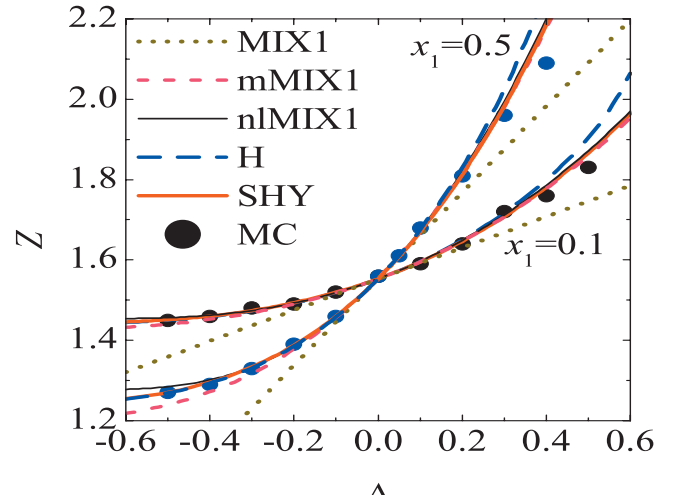
FIG. 7. Plot of the compressibility factor Z vs the nonadditivity parameter \Delta for a symmetric binary mixture of nonadditive hard spheres at \eta = \pi/30 and two different compositions. The dotted lines correspond to the original MIX1 theory, Eq. (3.3), the short-dashed lines correspond to the mMIX1 theory, Eq. (3.3) with Y_{ij}^M \rightarrow Y_{ij}^{mM} , the thin solid lines correspond to the nLMIX1 theory, Eq. (3.31), the long-dashed lines correspond to Hamad's proposal, Eq. (3.18), and the thick solid lines correspond to the SHY proposal, Eq. (3.24). The symbols are results from Monte Carlo simulations (Refs. 10 and 11).
