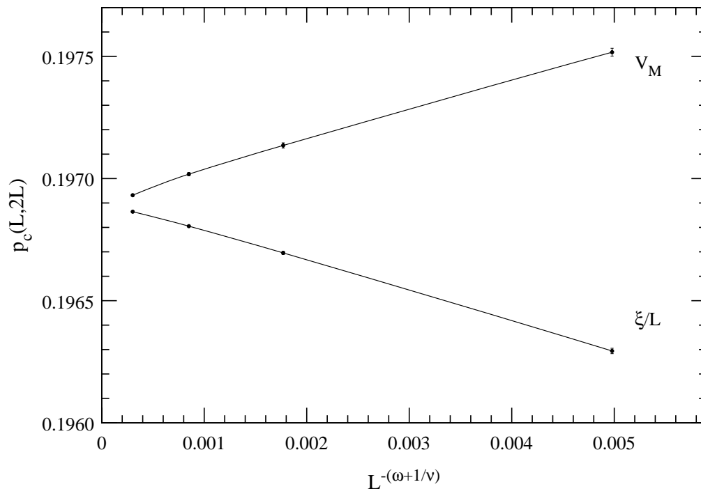
Figure 1: p_c(L, 2L) as a function of L^{-(\omega+1/\nu)} for the observables V_M and \xi/L .
