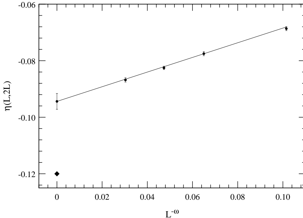
Figure 2: \eta(L, 2L) as a function of L^{-\omega} , where \omega is the corrections-to-scaling exponent, that we have fixed in this plot to 1.13 (see text for more details). The numerical value found in the literature, \eta = -0.12 , is also displayed.
