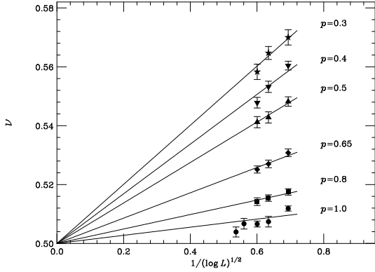
Figure 2. Exponent \nu estimation for (L, 2L) pairs. The solid lines are linear fits constrained to be \nu = 0.5 in the L \rightarrow \infty limit.
