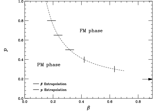
Figure 1. Phase diagram of the d = 4 site-diluted Ising model. The ticks are plotted at the simulated values along the extrapolation direction. The black arrow indicates the percolation limit.
