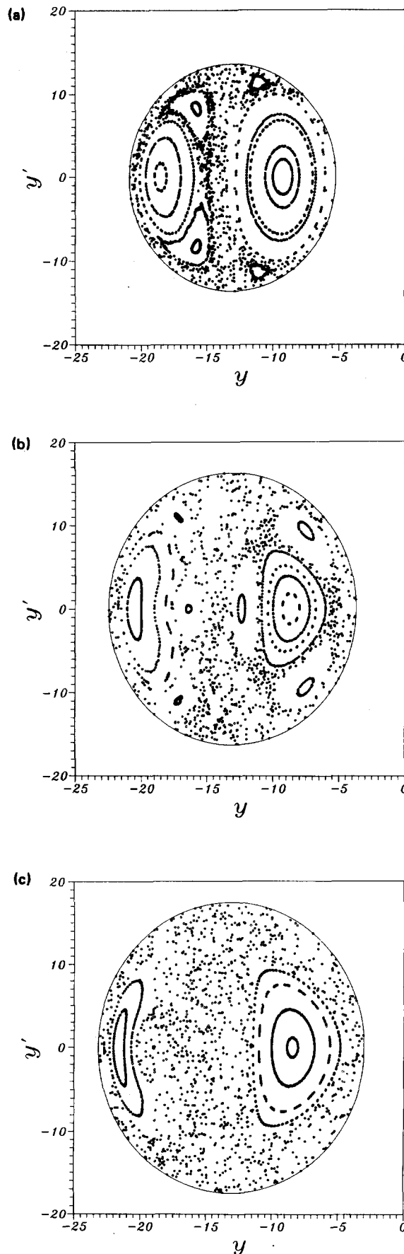
Fig. 3. Poincaré sections for different values of the energy: E/m = -20 J/kg for (a), E/m = 20 J/kg for (b) and E/m = 40 J/kg for (c). In all three cases \omega_m^2 = 3 \text{ s}^{-1} , \lambda = 3 . In every case the continuous curve marks the boundary of the energetically allowed region on the surface of section.
