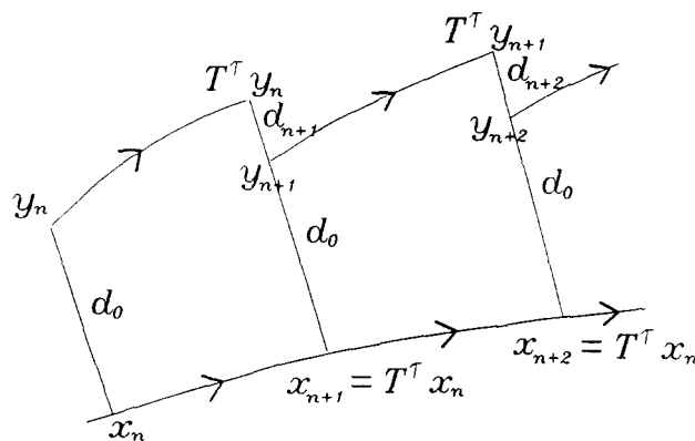
Fig. 4. Schematic description of the maximum Lyapunov exponent numerical computation. d_0 is the fiducial distance between the two nearby initial conditions x_0, y_0, y_n = T^T y_{n-1} is the n th point obtained in a numerical integration with time step \tau , with initial conditions y_{n-1} .
