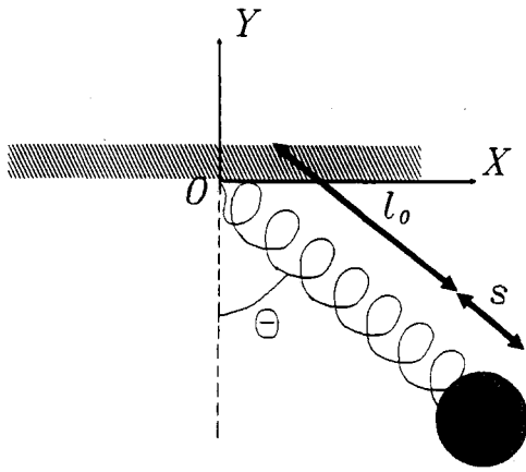
Fig. 1. The elastic pendulum.
